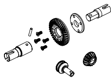
Starrachse hinten Fixed drive rear
