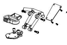
Frontrammer Front bumper
