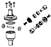
Differenzial vorne komplett Differential front complete
